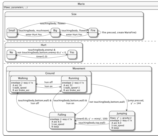
Figure 3: (Simplified) Super Mario as a hybrid automaton.
