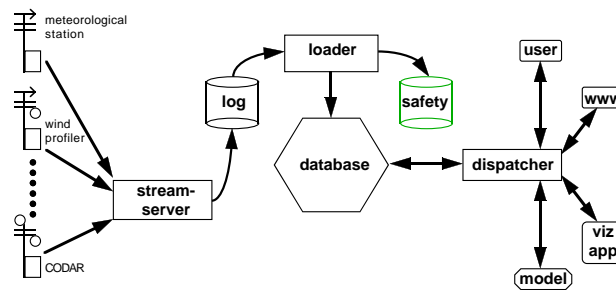
Figure 1: REINAS System Data Flow, Database Node View
