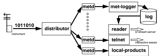
Figure 2: Instrument Node Data Flow
