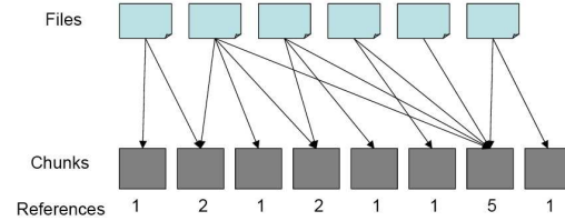
Figure 3. Inter-file dependencies
