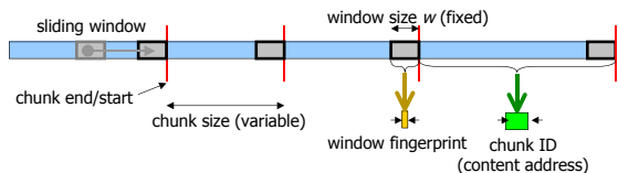
Figure 1. Sliding Window Technique
