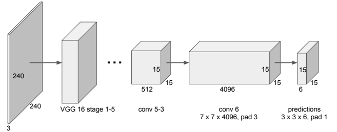
Figure 4. The structure of WordDetNet, shown here for N=15 and B=1 . Our experiments show the above configuration achieves the best result.
